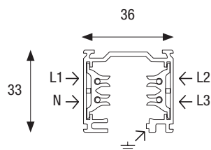
Binario trifase on-off. (*) 3-phase on-off track.
