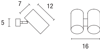
Wall 2x Spots
