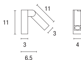
Square Wall mounting
